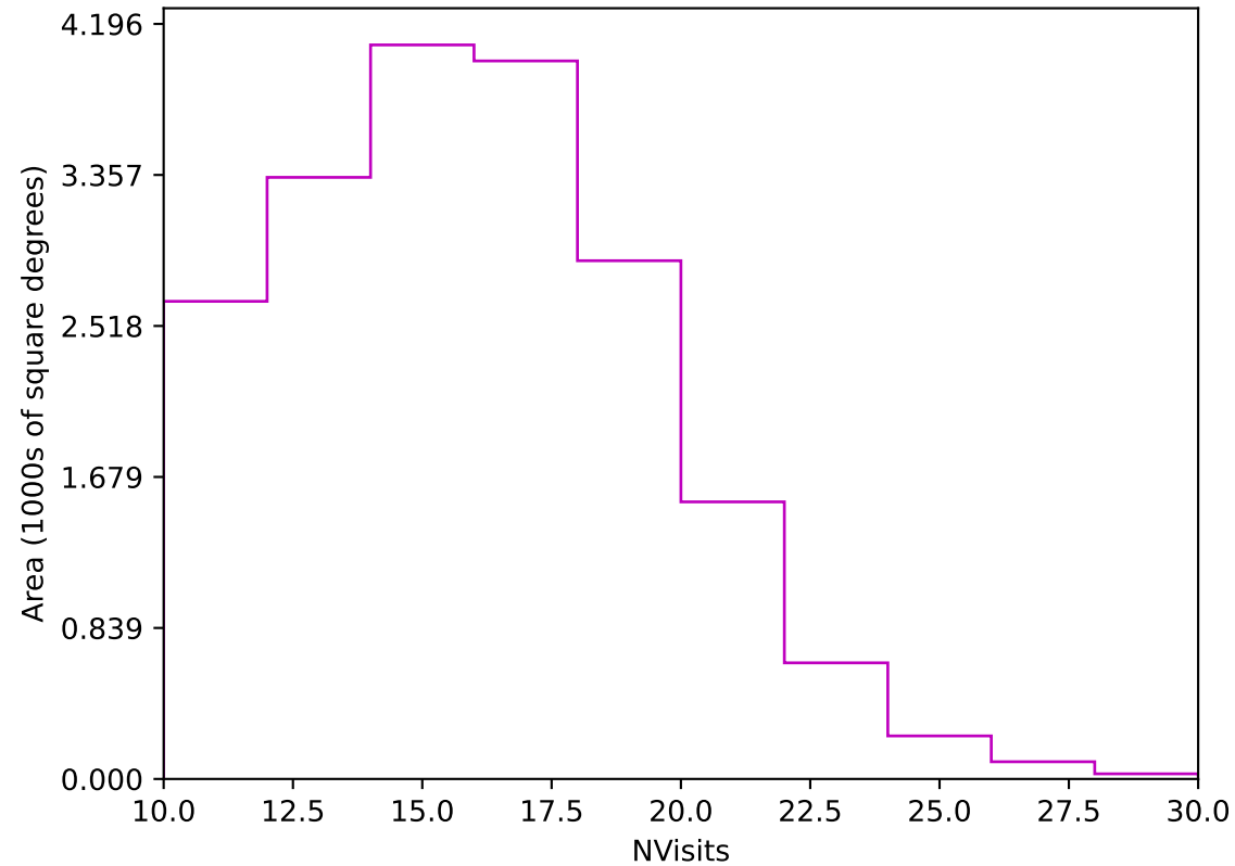
weather_cloudso30v3.4_10yrs Yr 1 z band: NVisits
