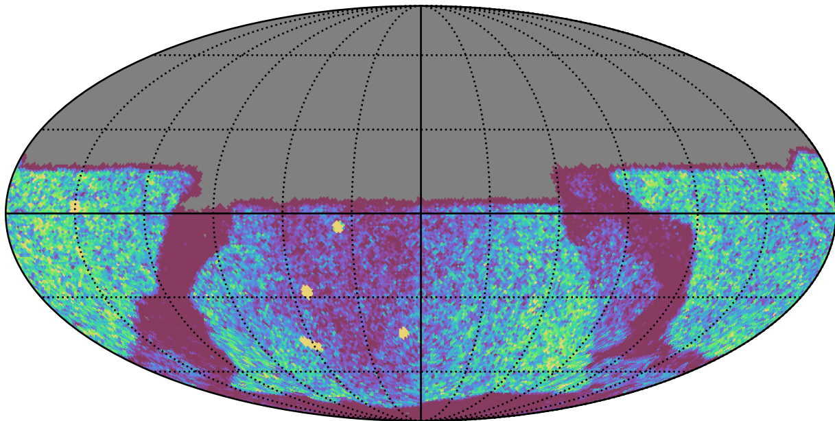
weather_cloudso30v3.4_10yrs Yr 1 y band: NVisits
