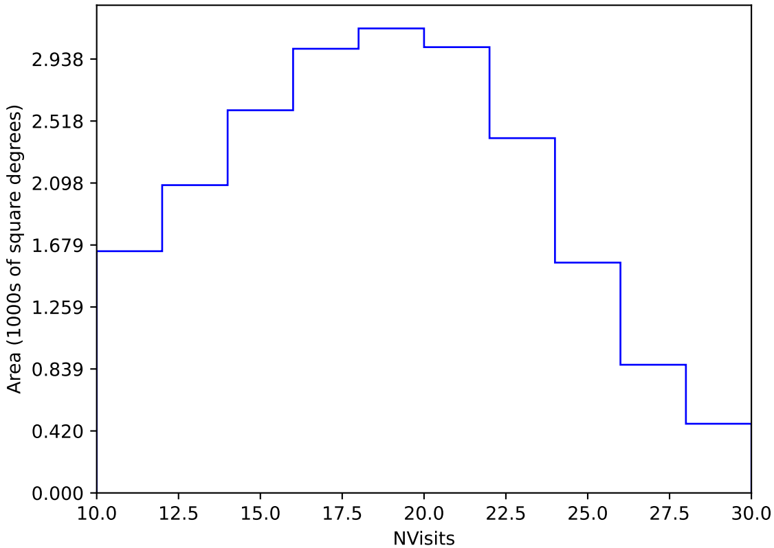
weather_cloudso30v3.4_10yrs Yr 1 y band: NVisits
