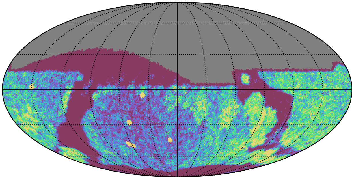
weather_cloudso30v3.4_10yrs Yr 1 r band: NVisits
