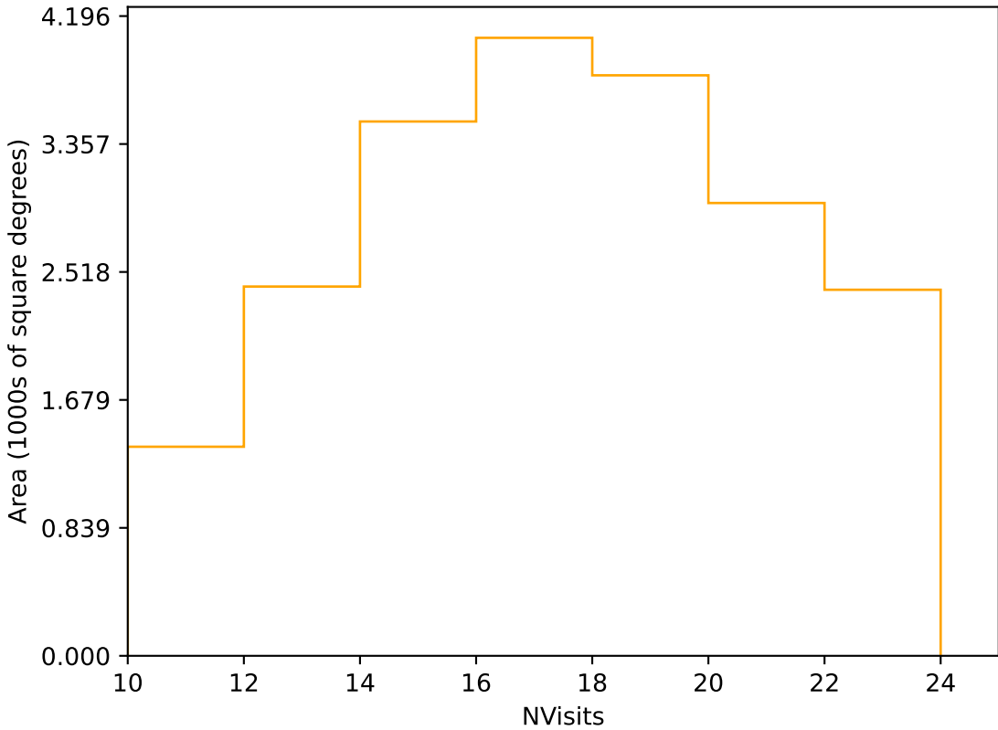
weather_cloudso30v3.4_10yrs Yr 1 r band: NVisits
