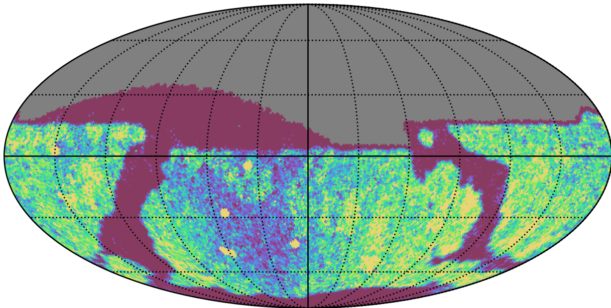
weather_cloudso30v3.4_10yrs Yr 1 i band: NVisits
