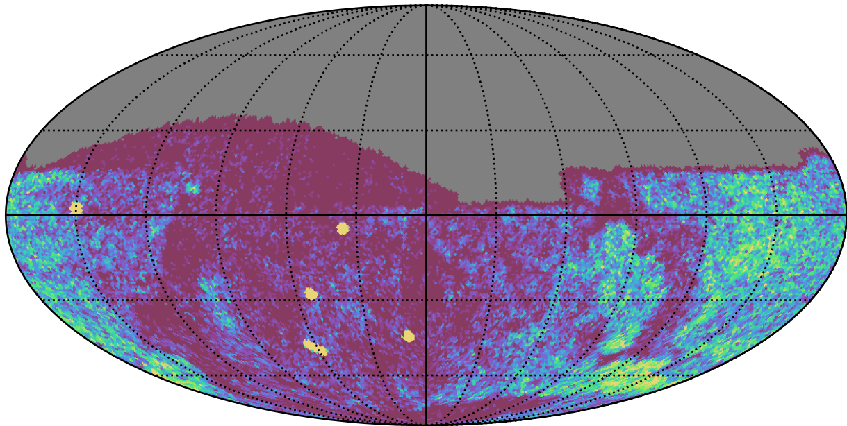
weather_cloudso30v3.4_10yrs Yr 1 g band: NVisits
