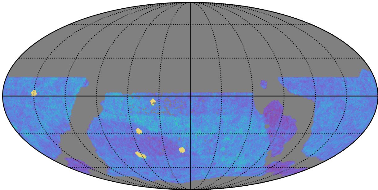
weather_cloudso30v3.4_10yrs WFD z band: NVisits
