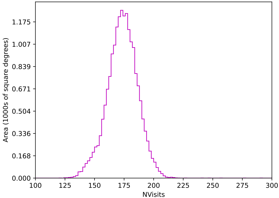
weather_cloudso30v3.4_10yrs WFD z band: NVisits
