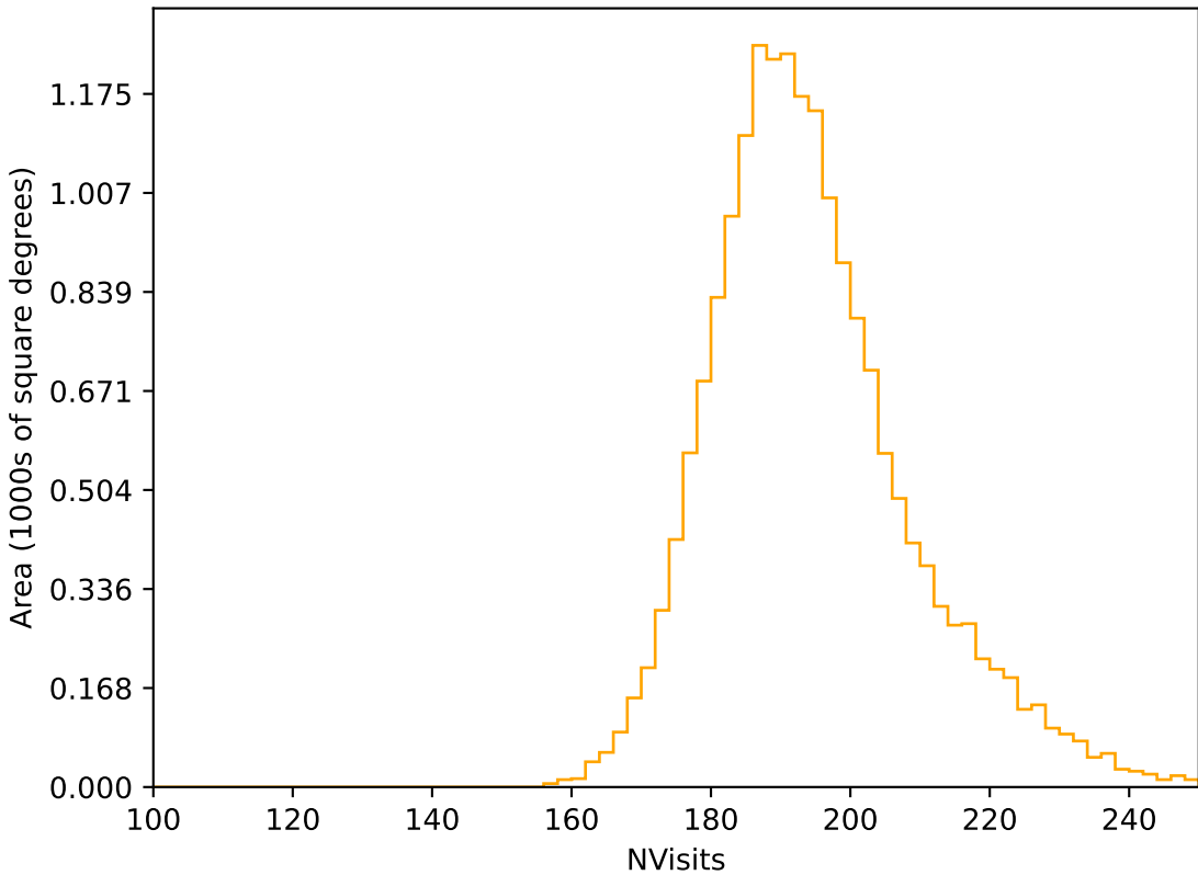
weather_cloudso30v3.4_10yrs WFD r band: NVisits
