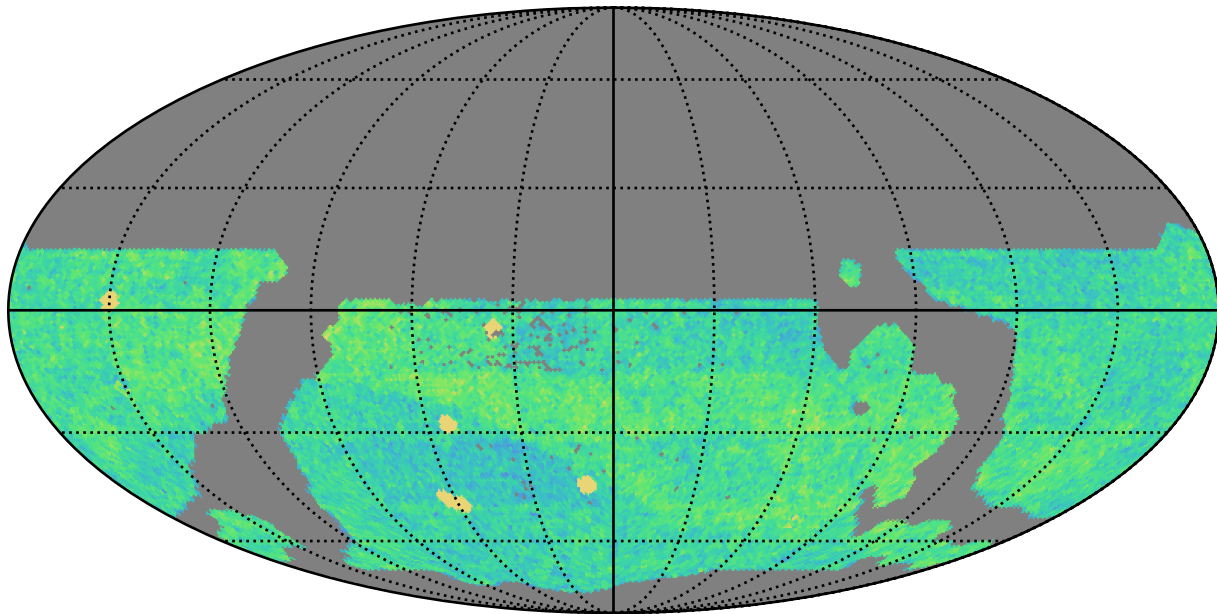
weather_cloudso30v3.4_10yrs WFD i band: NVisits
