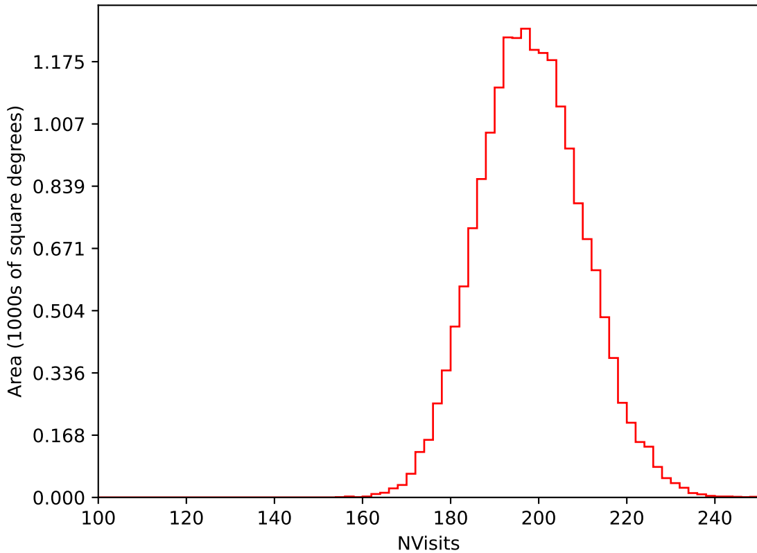
weather_cloudso30v3.4_10yrs WFD i band: NVisits
