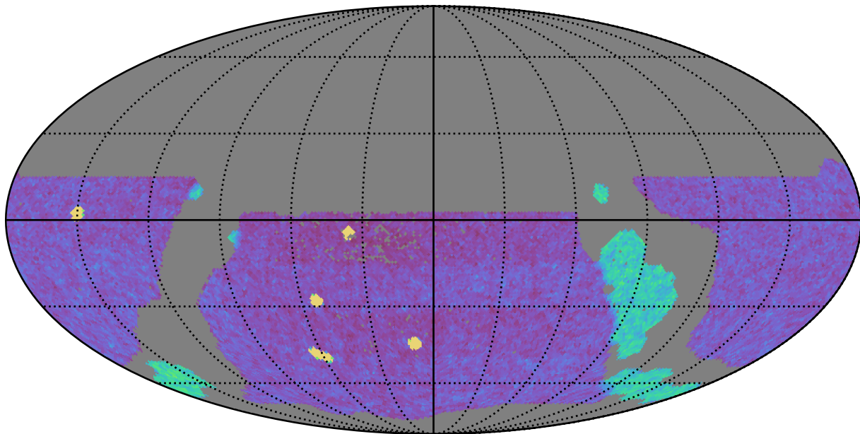
weather_cloudso30v3.4_10yrs WFD g band: NVisits
