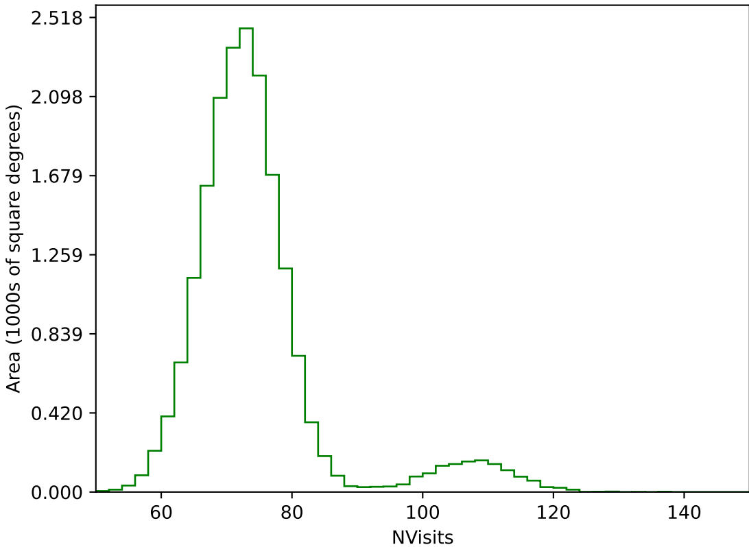
weather_cloudso30v3.4_10yrs WFD g band: NVisits
