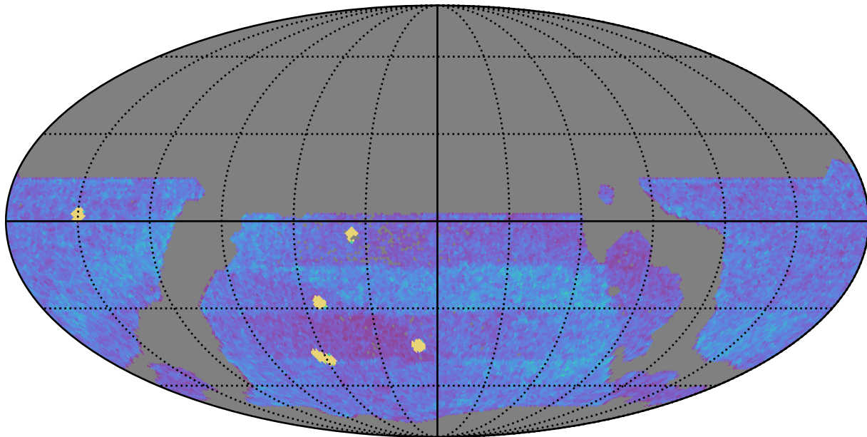
weather_cloudso30v3.4_10yrs WFD all bands: NVisits
