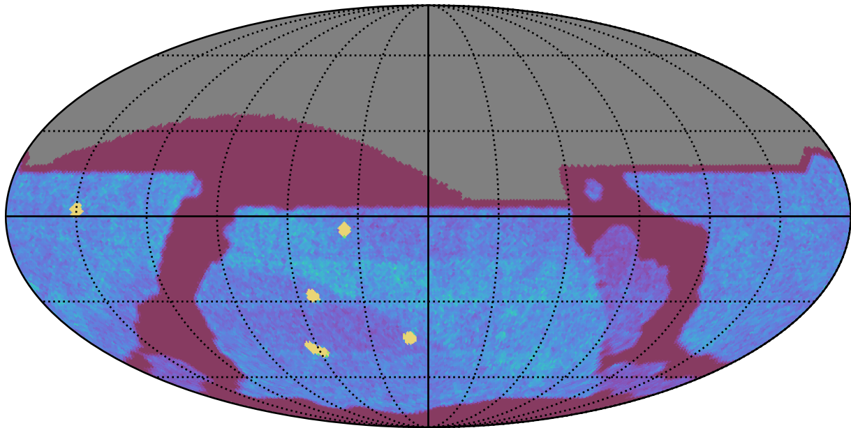
weather_cloudso30v3.4_10yrs All sky z band: NVisits
