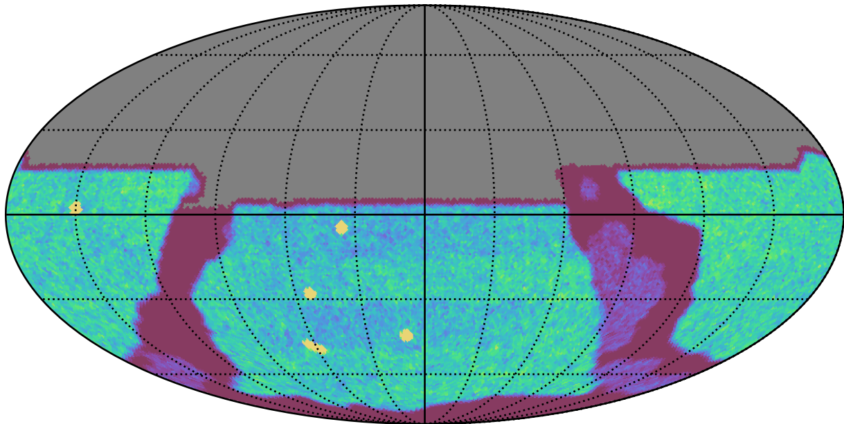
weather_cloudso30v3.4_10yrs All sky u band: NVisits
