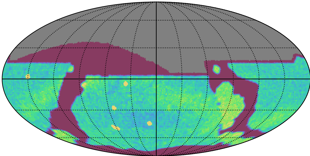
weather_cloudso30v3.4_10yrs All sky r band: NVisits
