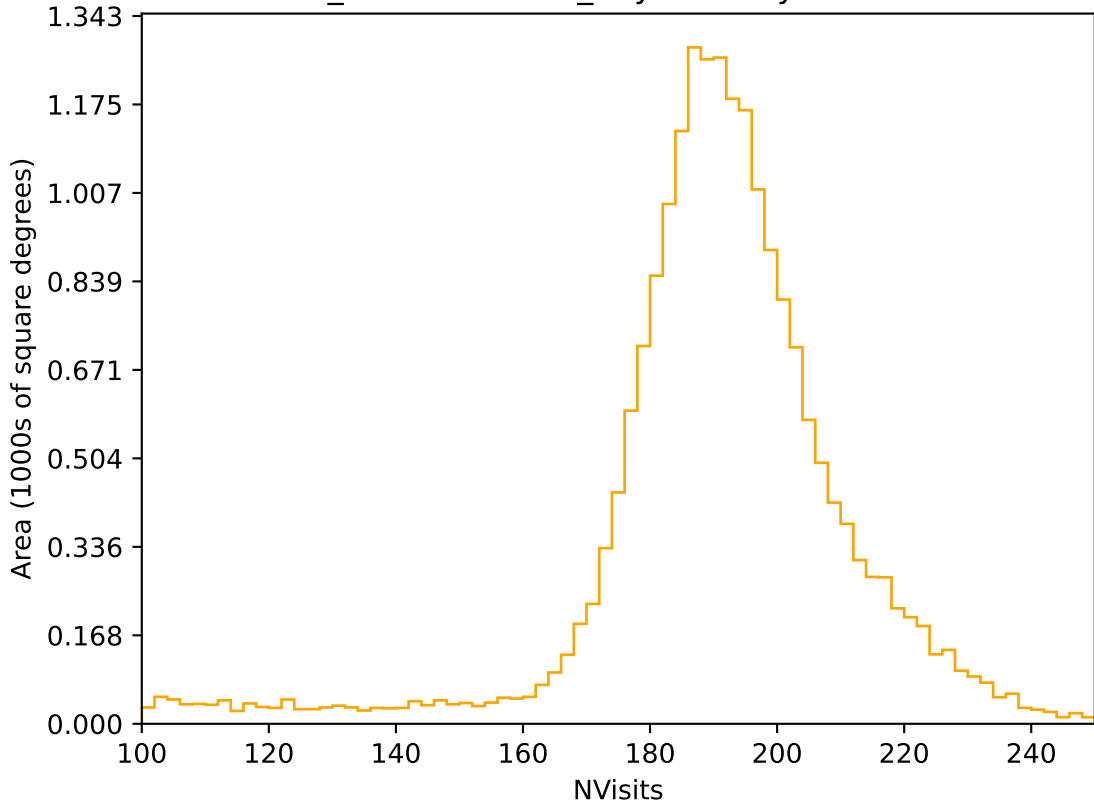
weather_cloudso30v3.4_10yrs All sky r band: NVisits
