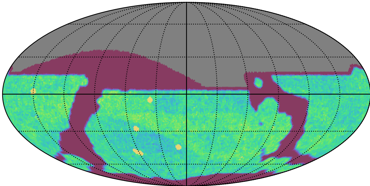
weather_cloudso30v3.4_10yrs All sky i band: NVisits
