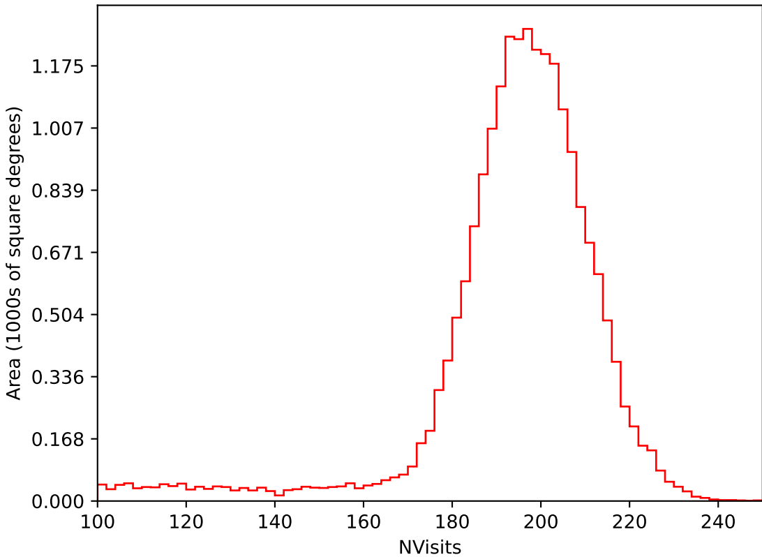
weather_cloudso30v3.4_10yrs All sky i band: NVisits
