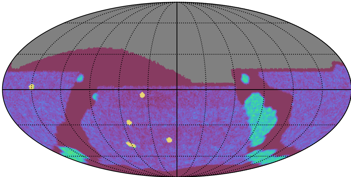
weather_cloudso30v3.4_10yrs All sky g band: NVisits
