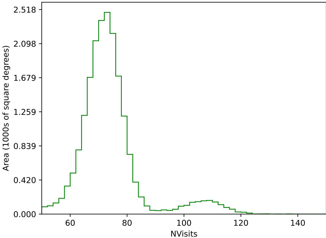
weather_cloudso30v3.4_10yrs All sky g band: NVisits
