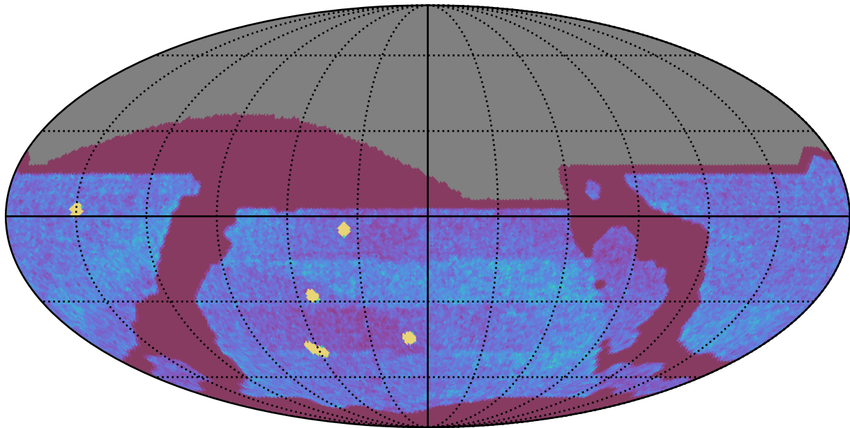
weather_cloudso30v3.4_10yrs All sky all bands: NVisits
