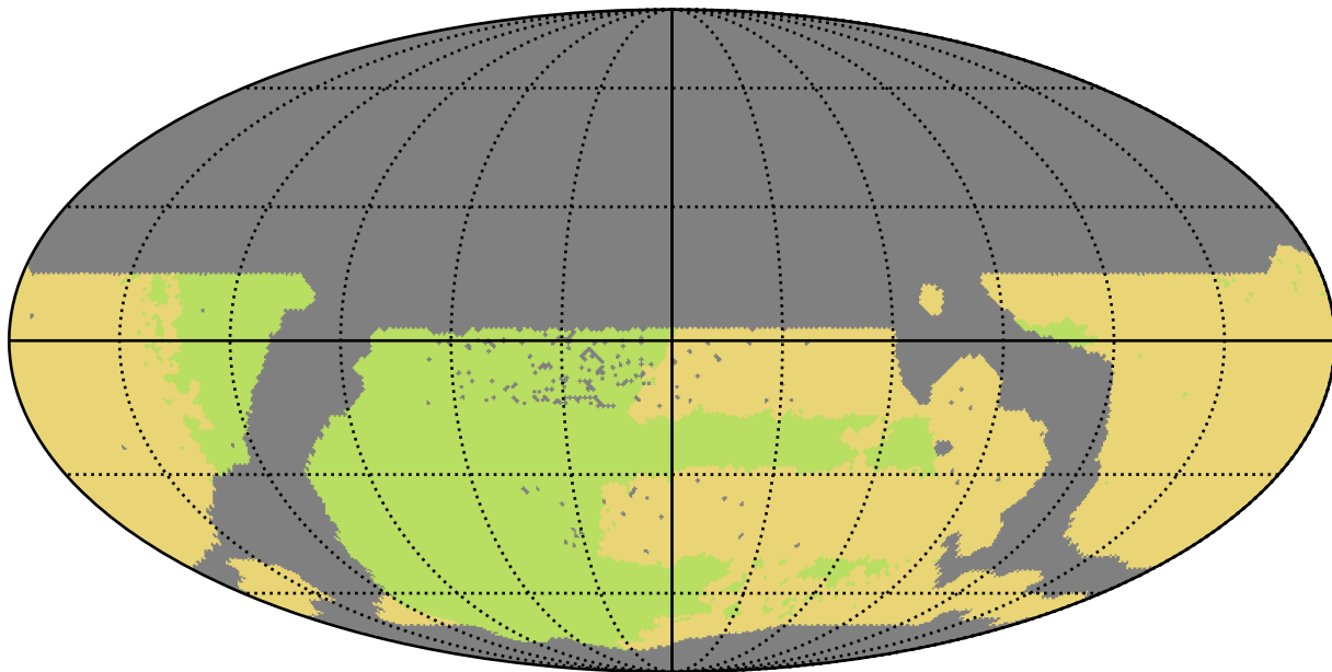
weather_cloudso30v3.4_10yrs WFD all bands: NSeasons
