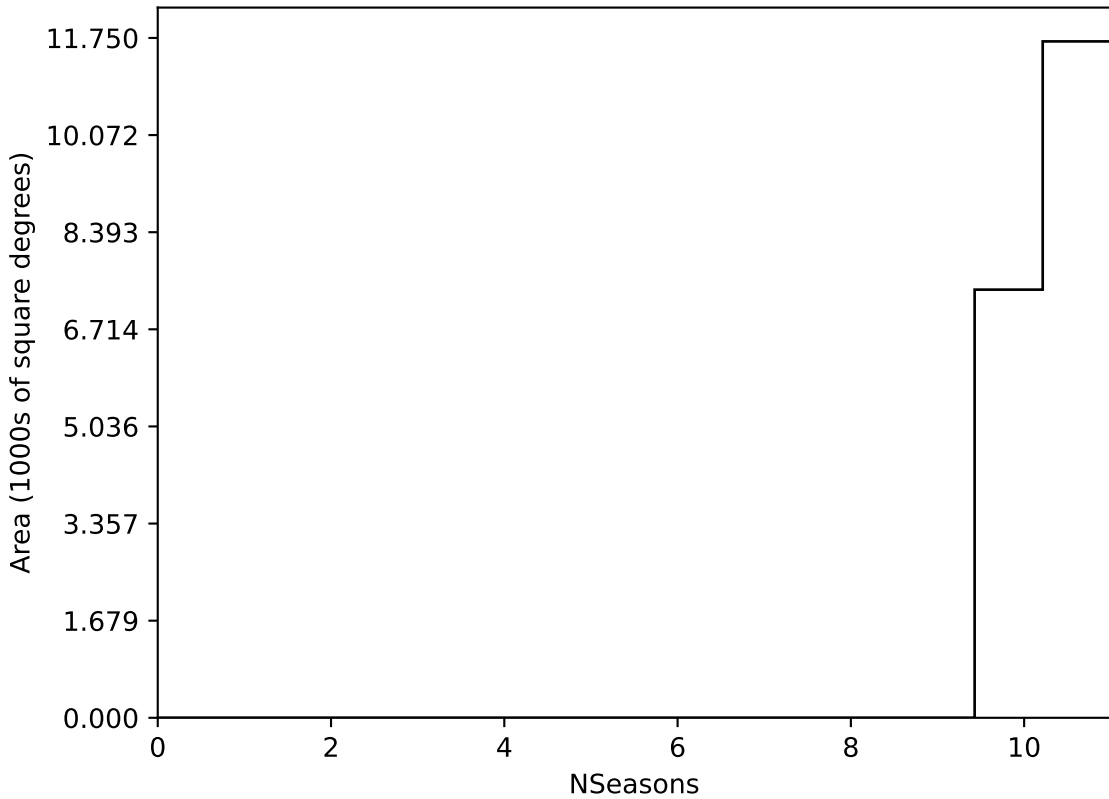
weather_cloudso30v3.4_10yrs WFD all bands: NSeasons
