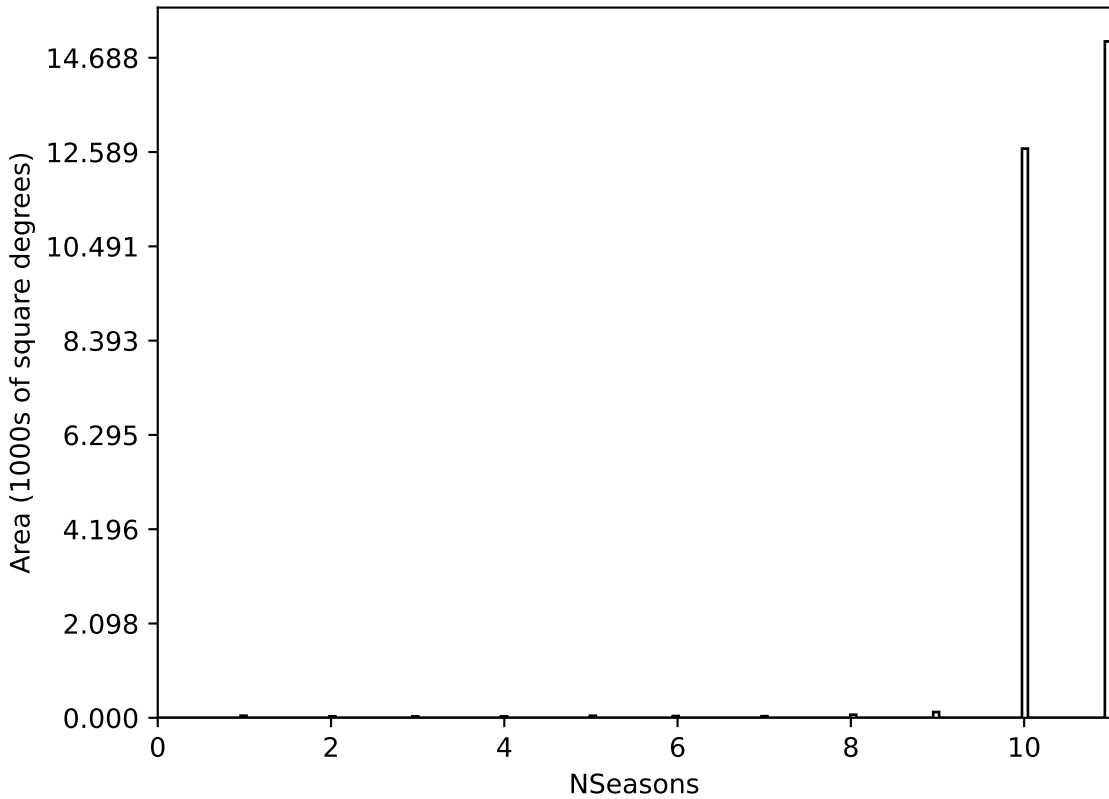
weather_cloudso30v3.4_10yrs All sky all bands: NSeasons
