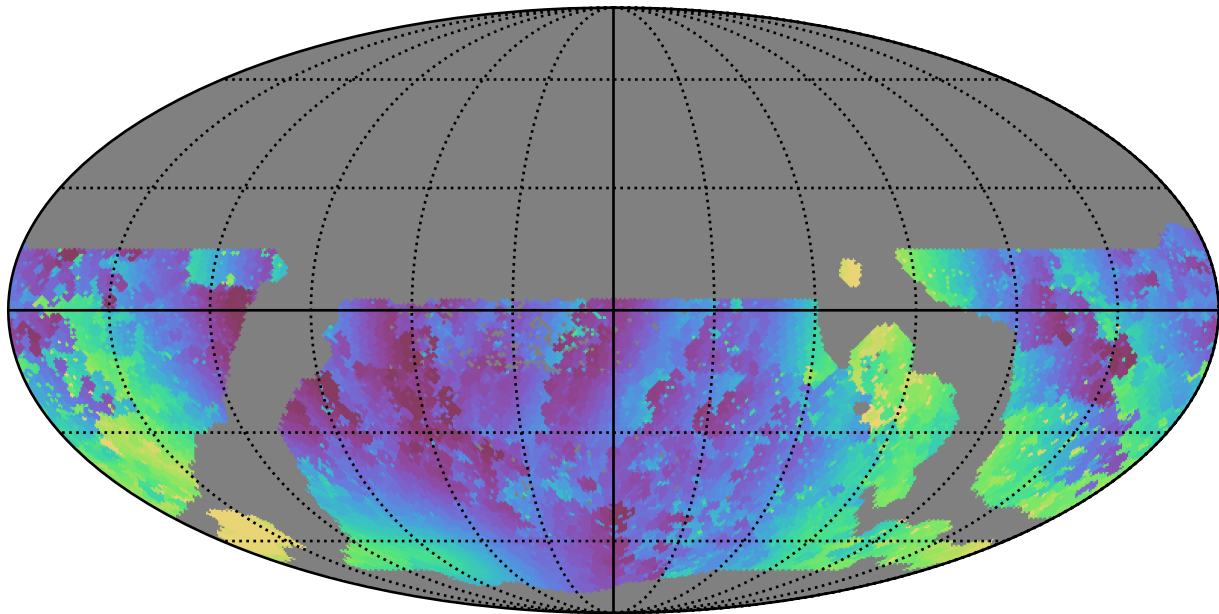
weather_cloudso30v3.4_10yrs WFD u band: Min solarElong
