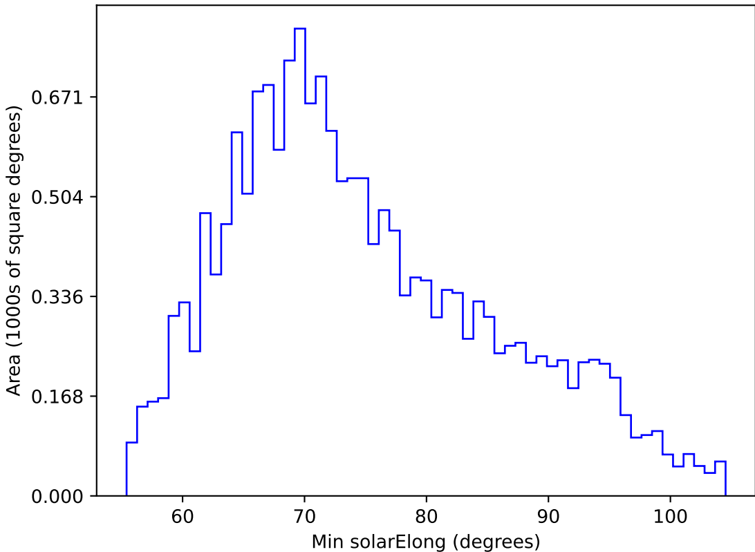
weather_cloudso30v3.4_10yrs WFD u band: Min solarElong
