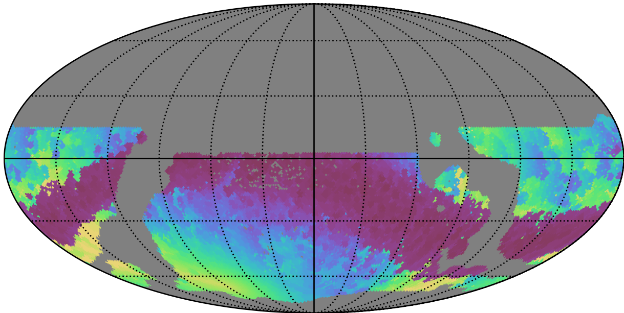
weather_cloudso30v3.4_10yrs WFD r band: Min solarElong
