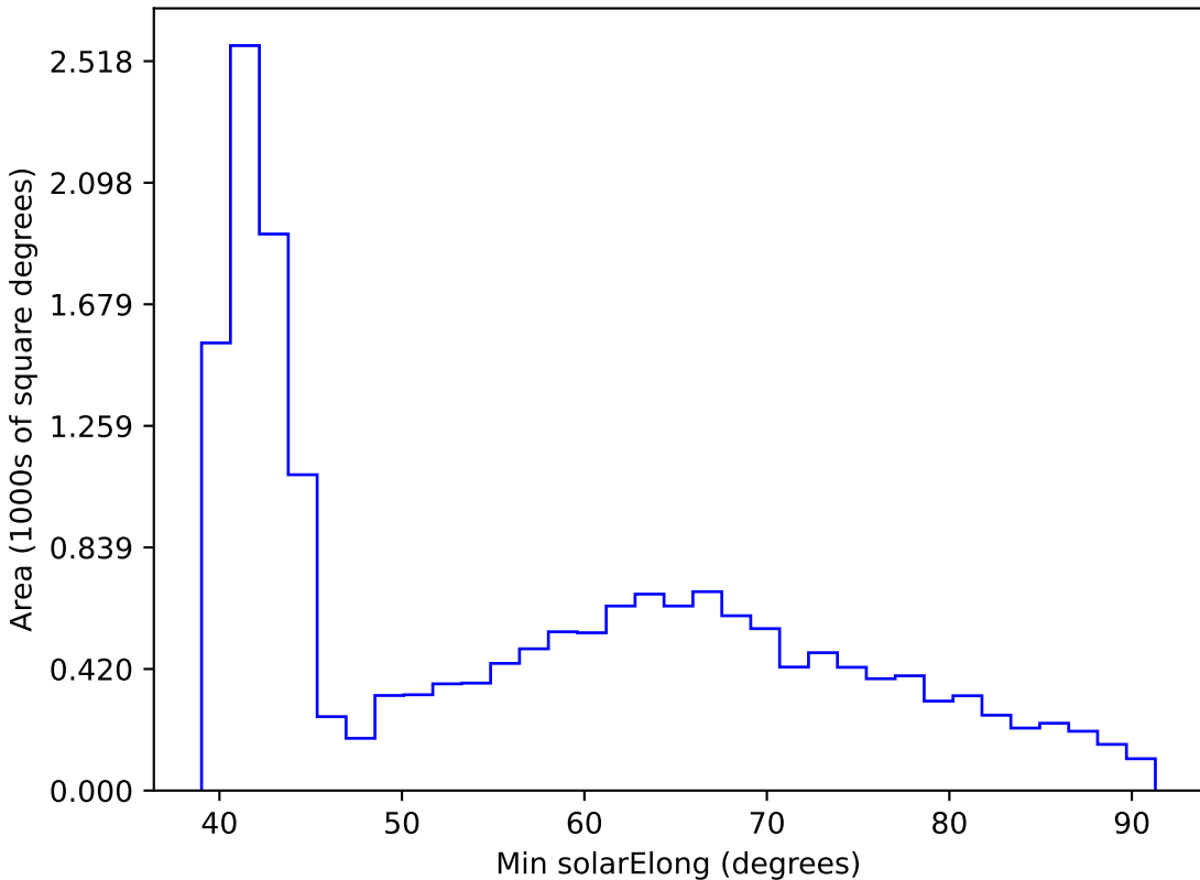
weather_cloudso30v3.4_10yrs WFD r band: Min solarElong
