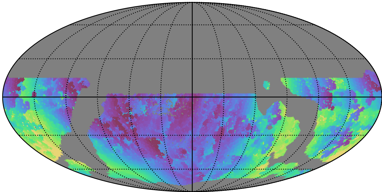
weather_cloudso30v3.4_10yrs WFD g band: Min solarElong
