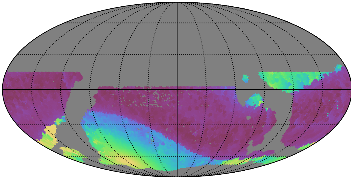
weather_cloudso30v3.4_10yrs WFD all bands: Min solarElong
