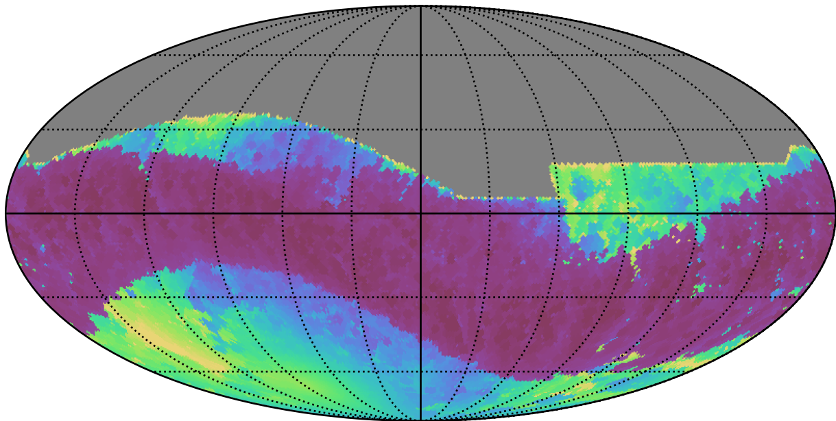
weather_cloudso30v3.4_10yrs All sky z band: Min solarElong
