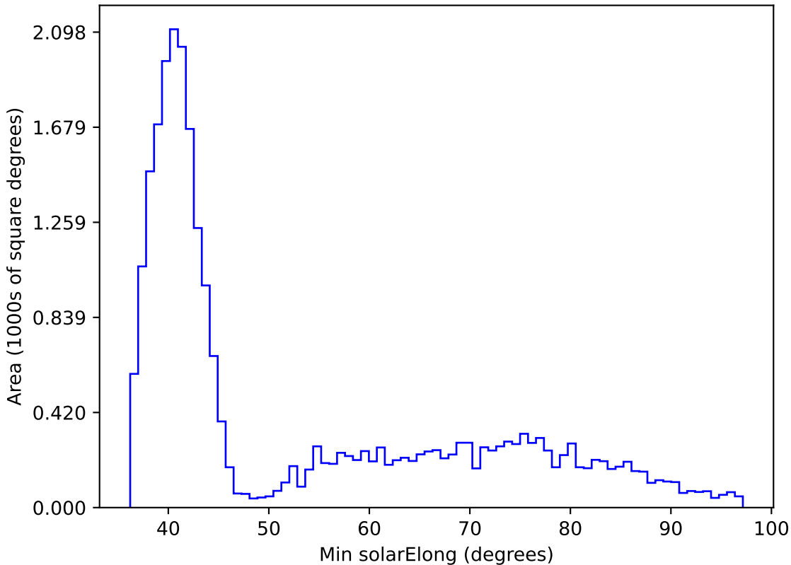
weather_cloudso30v3.4_10yrs All sky z band: Min solarElong
