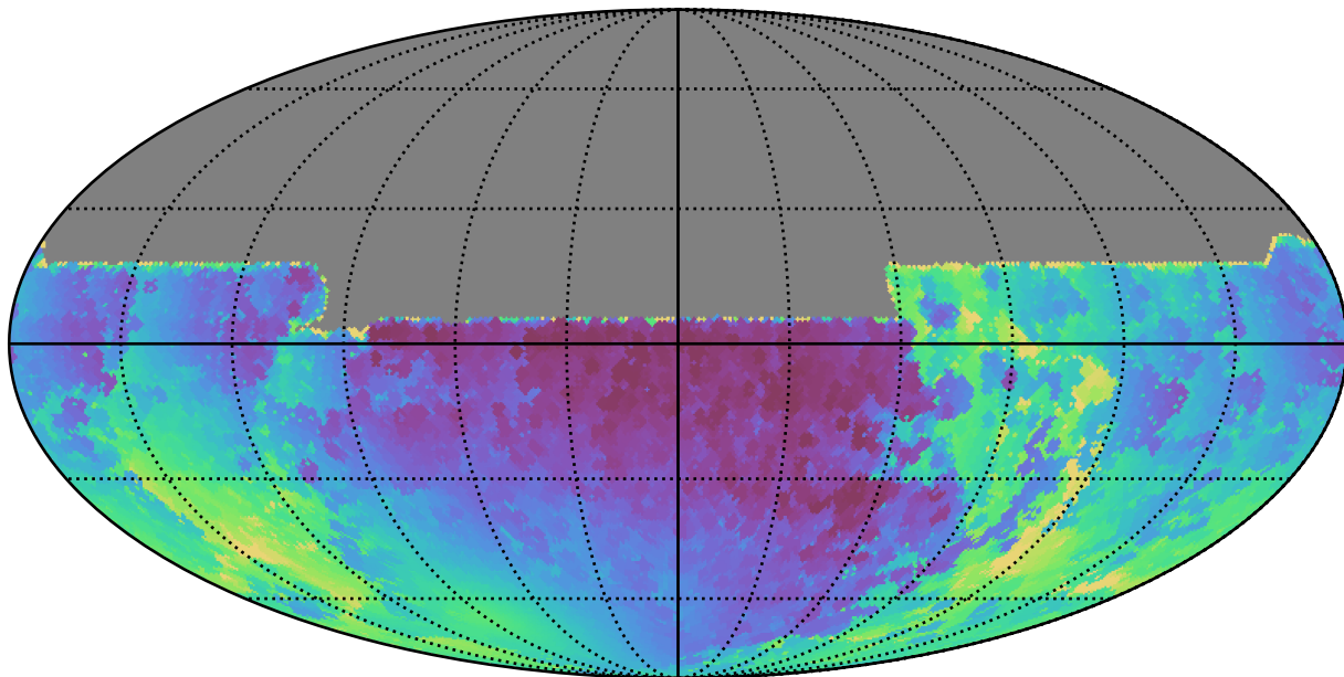
weather_cloudso30v3.4_10yrs All sky y band: Min solarElong
