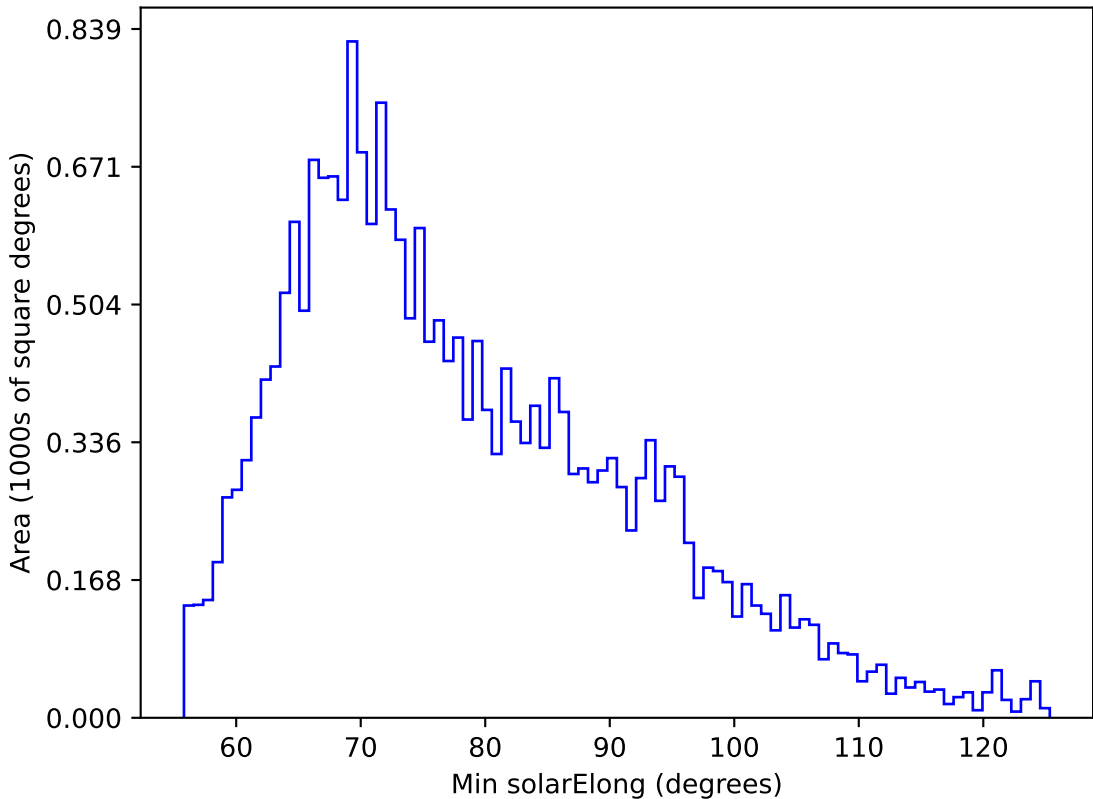
weather_cloudso30v3.4_10yrs All sky u band: Min solarElong
