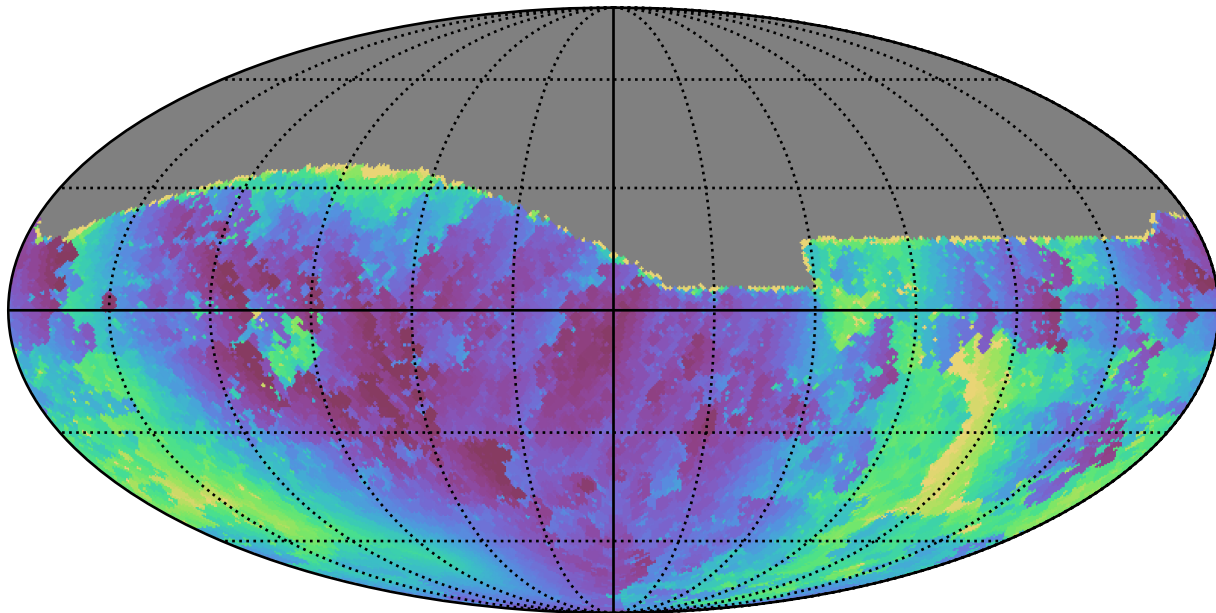
weather_cloudso30v3.4_10yrs All sky g band: Min solarElong
