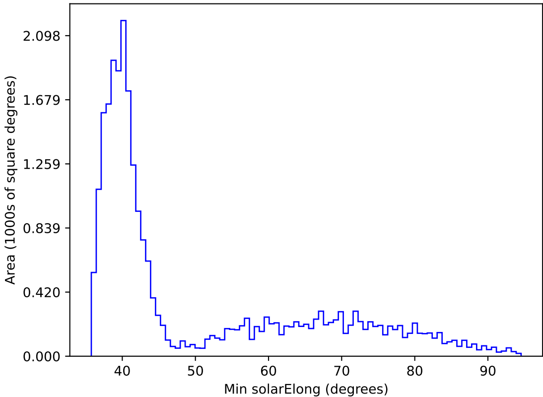
weather_cloudso30v3.4_10yrs All sky all bands: Min solarElong
