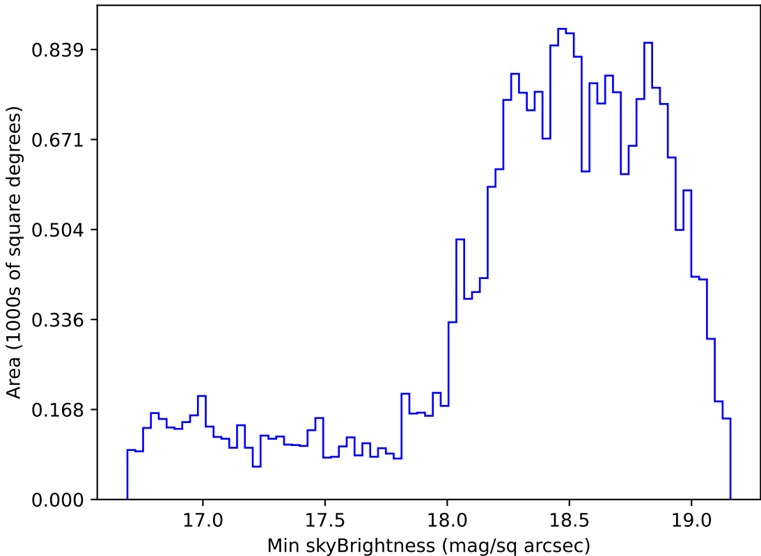
weather_cloudso30v3.4_10yrs Yr 1 z band: Min skyBrightness
