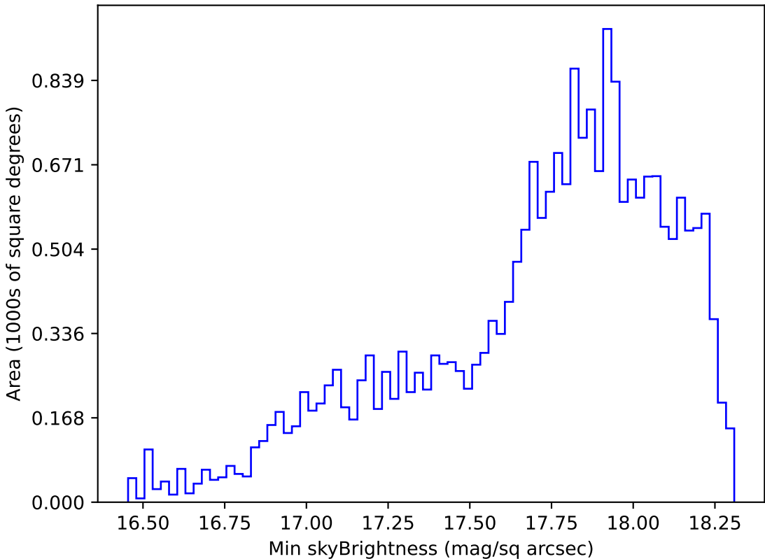
weather_cloudso30v3.4_10yrs Yr 1 y band: Min skyBrightness
