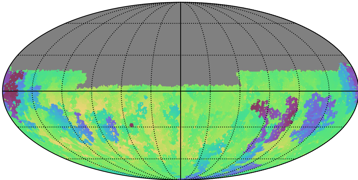
weather_cloudso30v3.4_10yrs Yr 1 u band: Min skyBrightness
