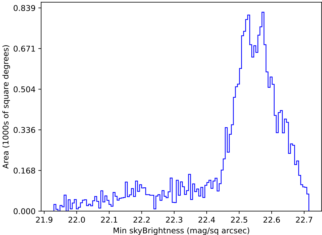
weather_cloudso30v3.4_10yrs Yr 1 u band: Min skyBrightness
