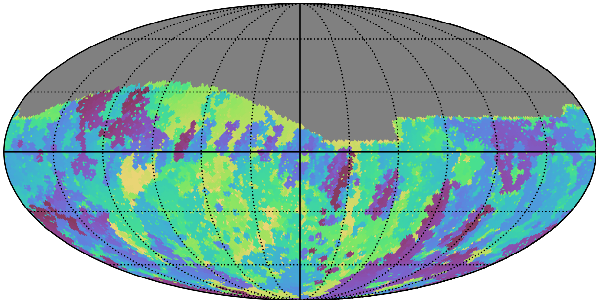
weather_cloudso30v3.4_10yrs Yr 1 r band: Min skyBrightness
