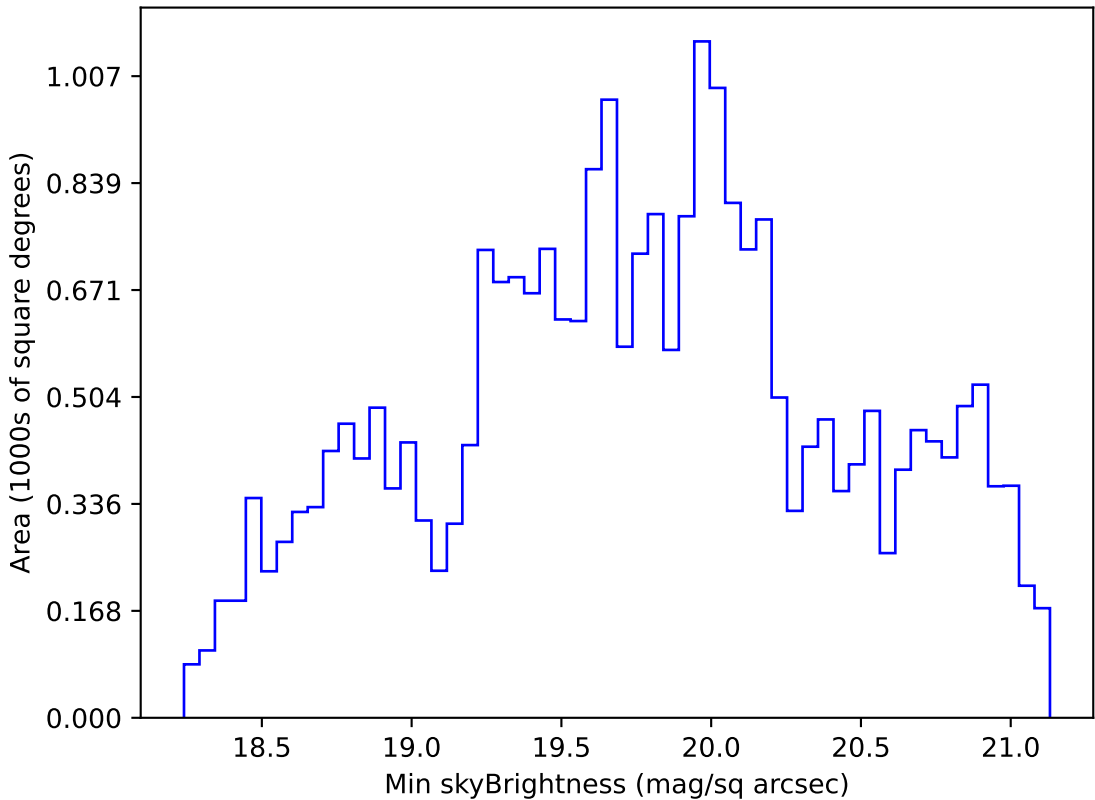
weather_cloudso30v3.4_10yrs Yr 1 r band: Min skyBrightness
