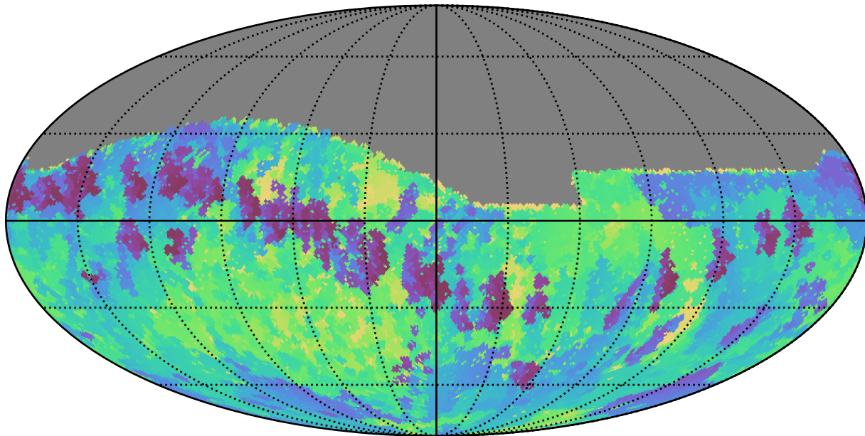
weather_cloudso30v3.4_10yrs Yr 1 i band: Min skyBrightness
