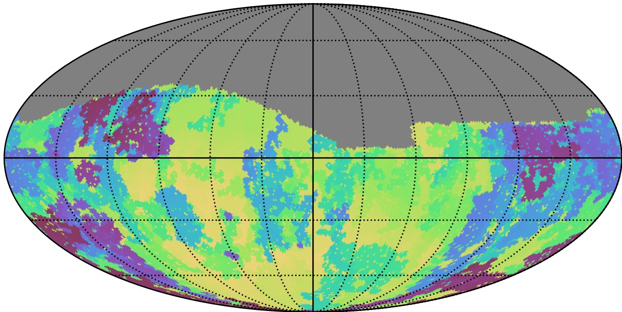
weather_cloudso30v3.4_10yrs Yr 1 g band: Min skyBrightness
