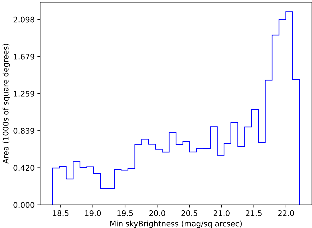
weather_cloudso30v3.4_10yrs Yr 1 g band: Min skyBrightness
