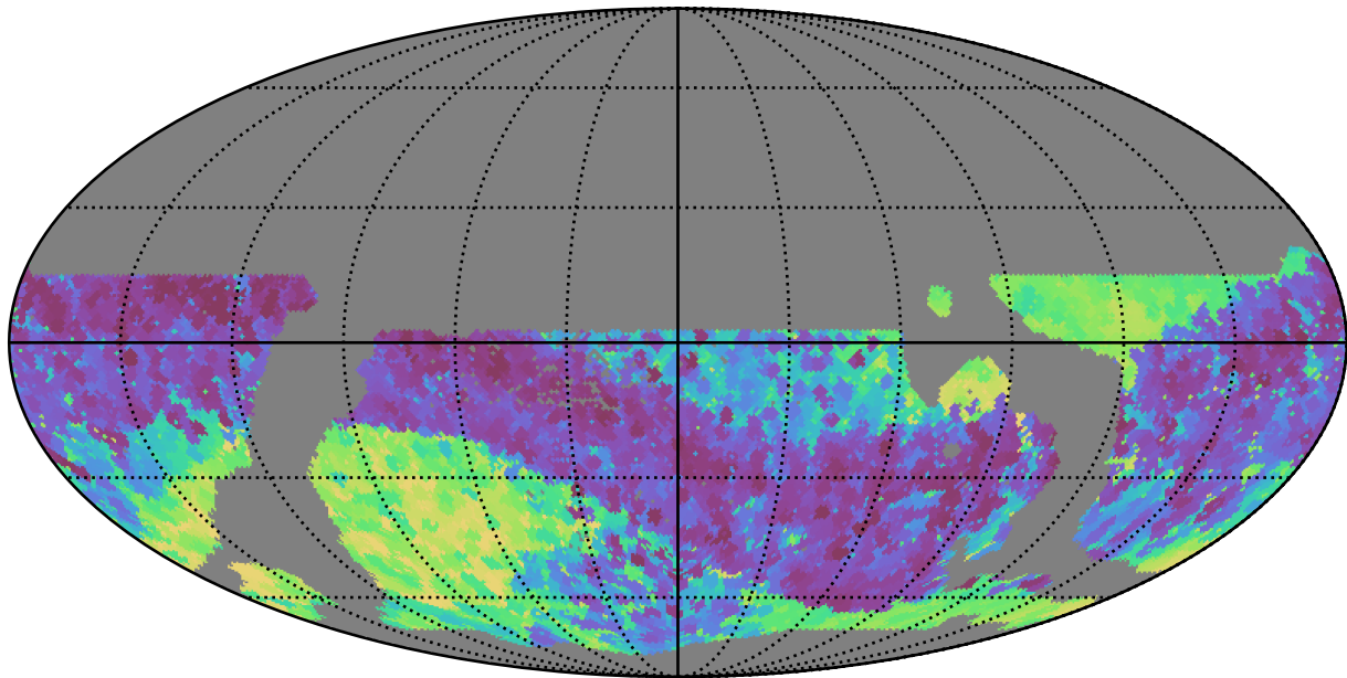
weather_cloudso30v3.4_10yrs WFD z band: Min skyBrightness
