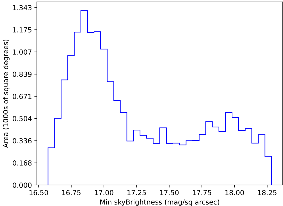
weather_cloudso30v3.4_10yrs WFD z band: Min skyBrightness
